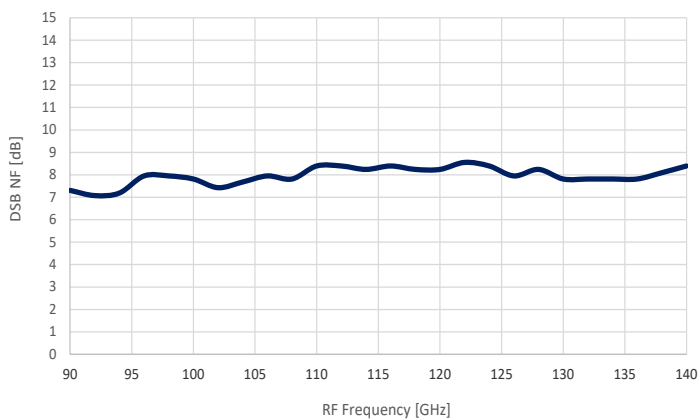
Typical DSB Noise Figure vs RF Frequency
