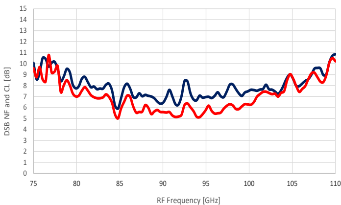
Typical DSB Noise Figure and Conversion Loss vs RF Frequency
