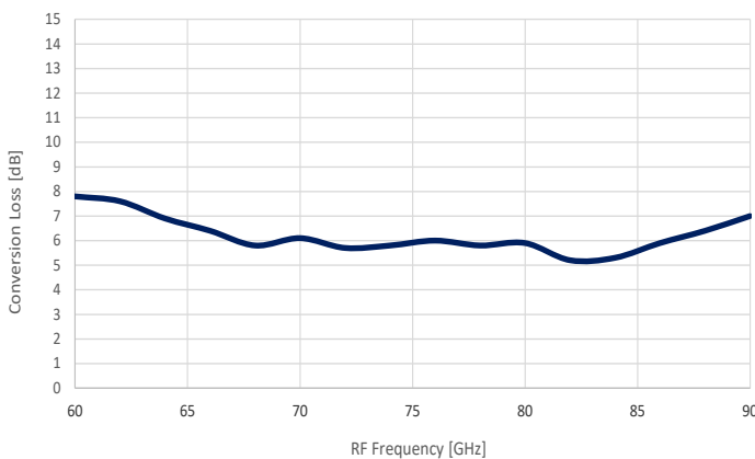
Typical Conversion Loss vs RF Frequency
