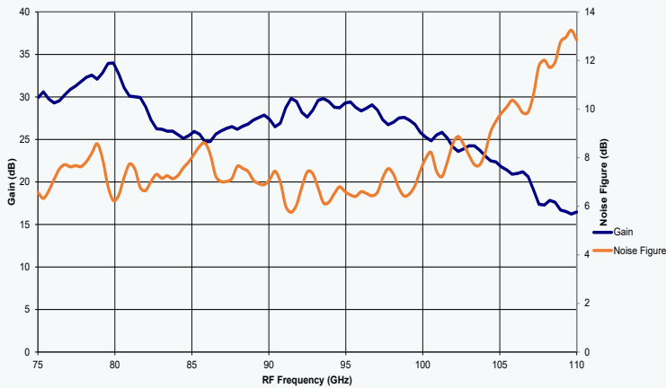
Gain & Noise Figure v RF Frequency
