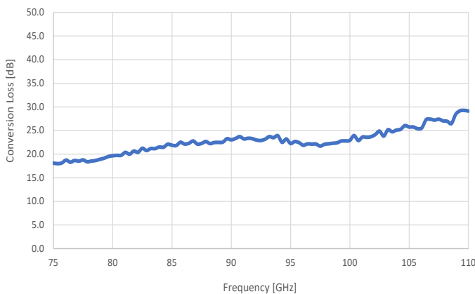
Typical Conversion Loss vs Frequency
